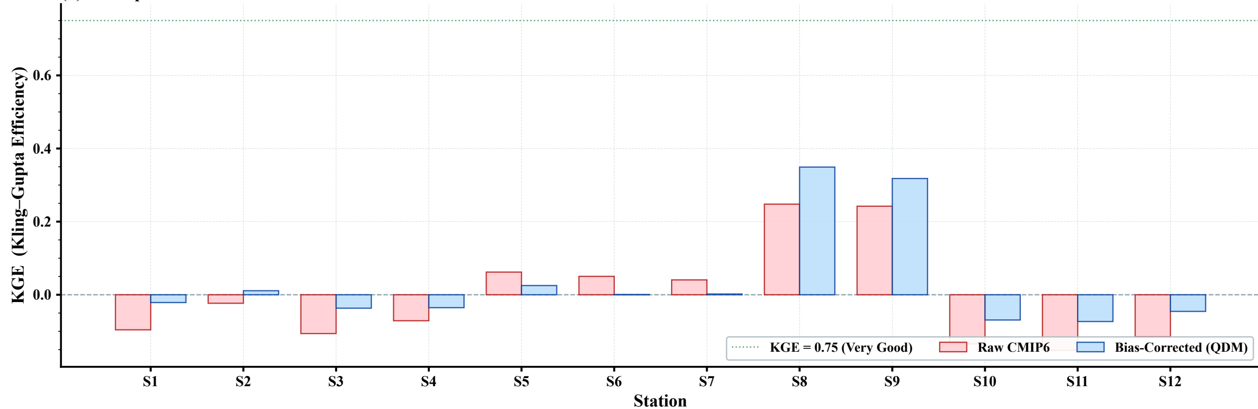
(b) KGE per Station — Ensemble Mean: Raw vs Bias-Corrected
