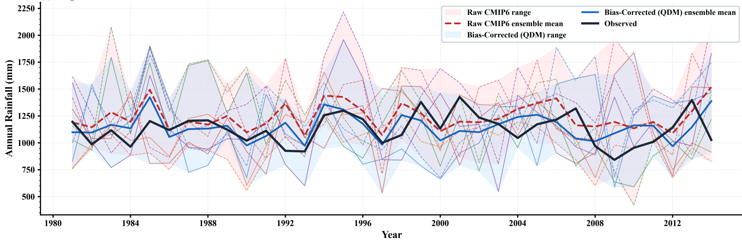
(a) Regional Mean Annual Rainfall — All Stations
